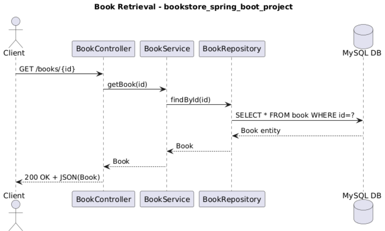
Figure 12: Sequence Diagram
